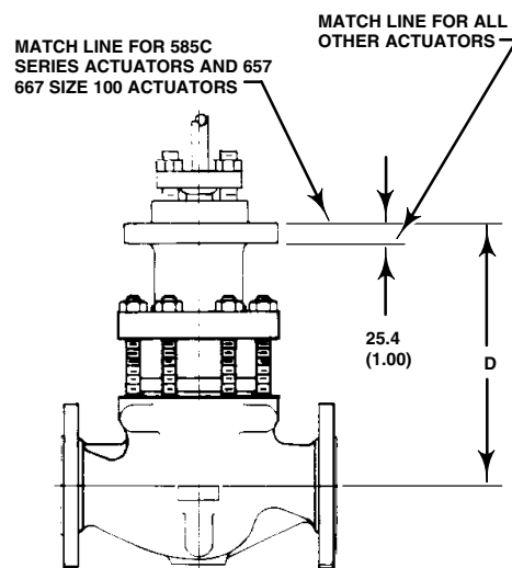
Figure 9. Non-Standard Dimensions (Cavitrol® III Two-Stage Trims Only) (also see tables 6 and 7)
