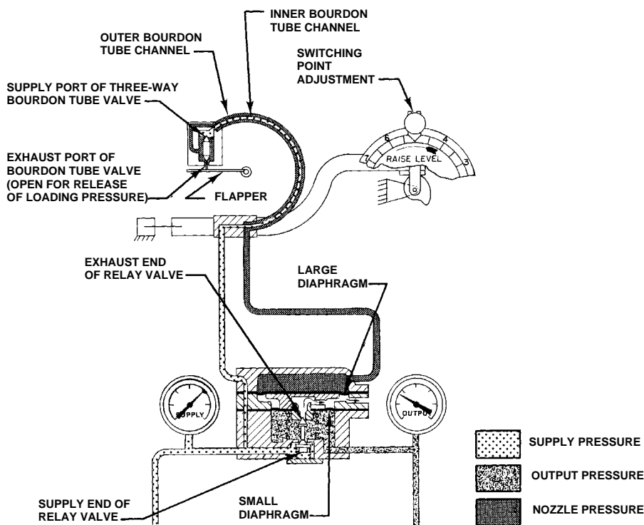
Figure 8. Schematic of Reverse-Acting 2503R Controller
