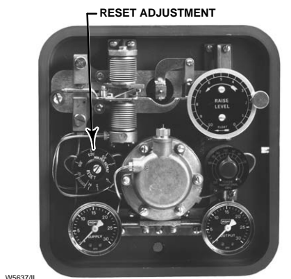
DETAIL OF DIRECT ACTING 2502 PROPORTIONAL-PLUS RESET CONTROLLER
