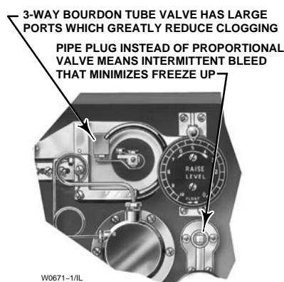
DETAIL OF REVERSE-ACTING 2503R ON-OFF CONTROLLER
