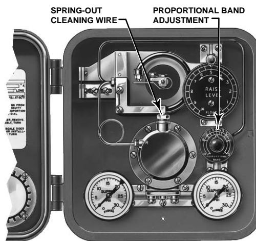
DIRECT-ACTING 2500 CONTROLLER
