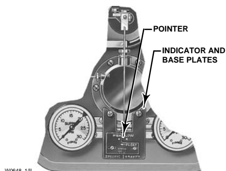
INDICATOR ASSEMBLY DETAIL
