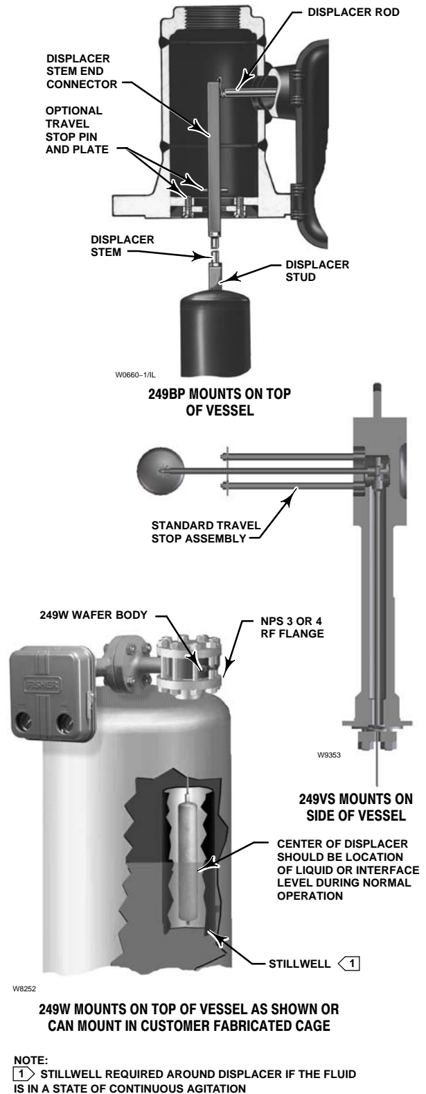
Figure 4. Typical Cageless Sensors
